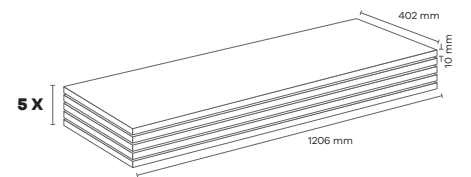
Panel / Paket: 5 Adet Paket: 2,424 m 2 ~21 kg
