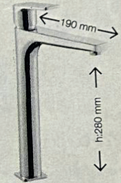
15680151 Azure Tall Basin Mixer Monoblock Body
